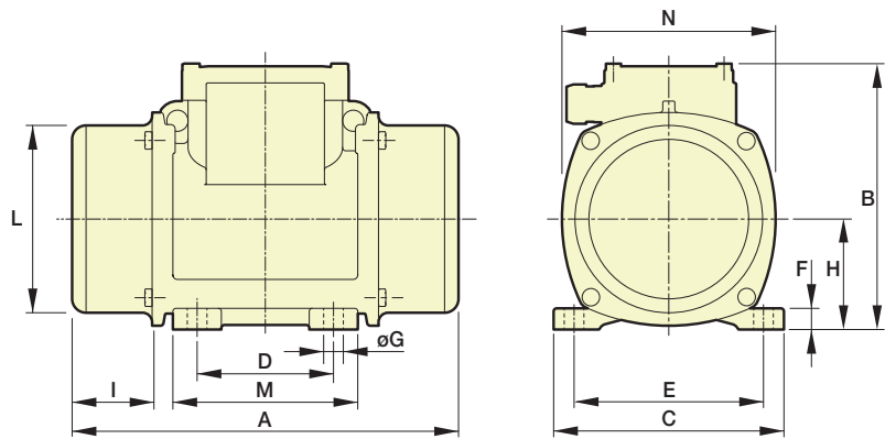
DIMENSIONAL SPECIFICATIONS (mm)
